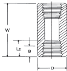
Coupling
